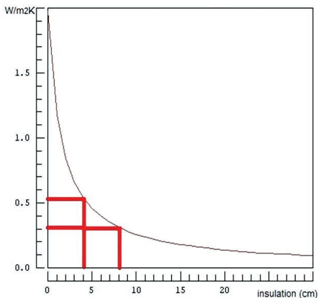
U-Value with and without StoTherm
